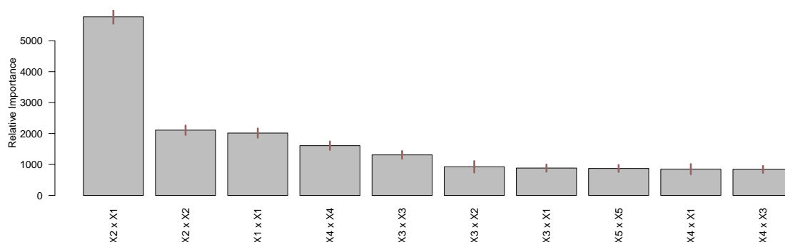
Figure 10: The top 10 average variable interaction counts (termed “relative importance”) in the default bartMachine model for the Friedman function data averaged over 25 model constructions. The segments atop the bars represent 95% confidence intervals.
